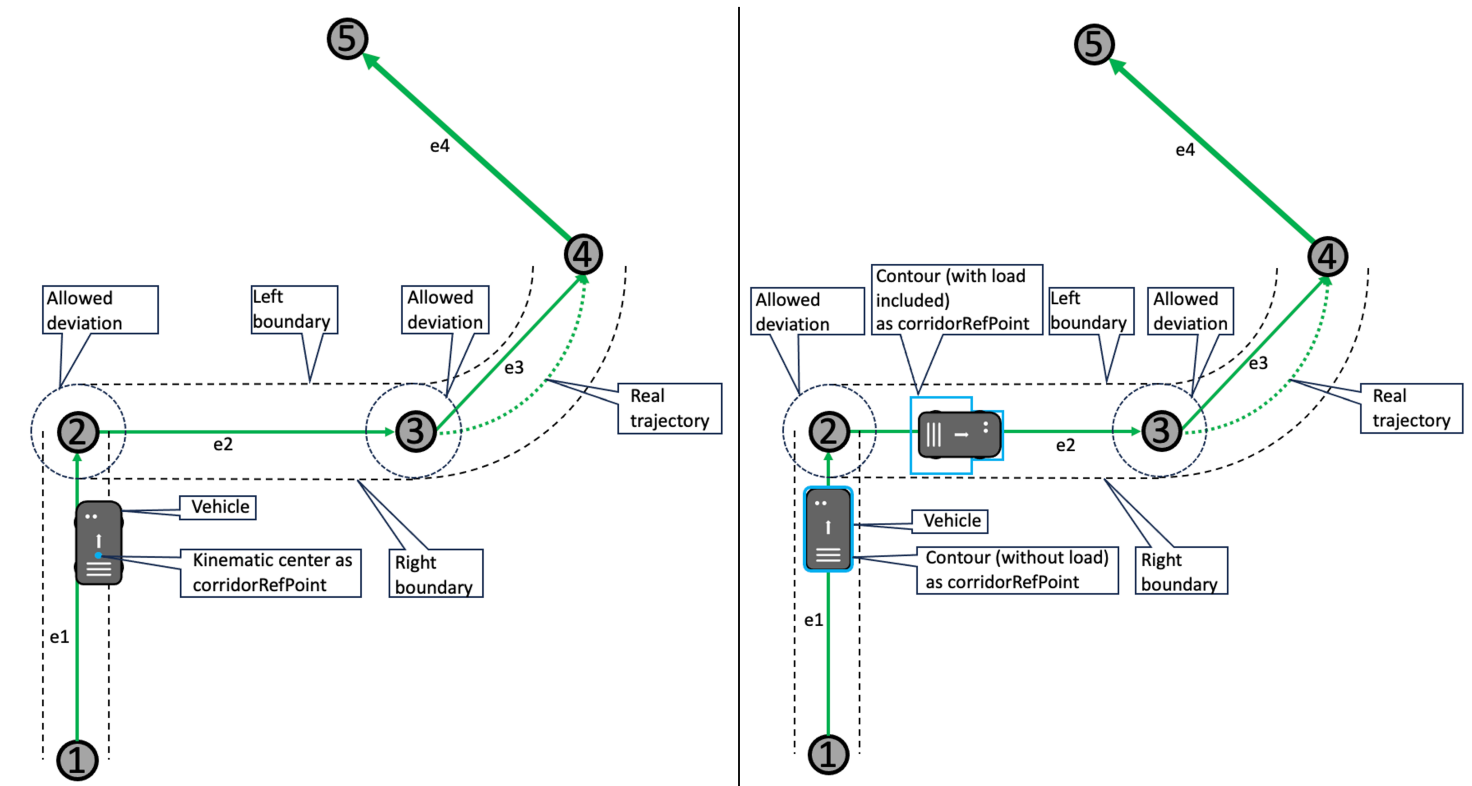
Figure 10 Edges with a corridor attribute that defines the left and right boundaries within which a vehicle is allowed to deviate from its predefined trajectory to avoid obstacles. On the left, the kinematic center defines the allowed deviation, while on the right, the contour of the vehicle, possibly extended by the load, defines the allowed deviation. This is defined by the corridorRefPoint parameter.
