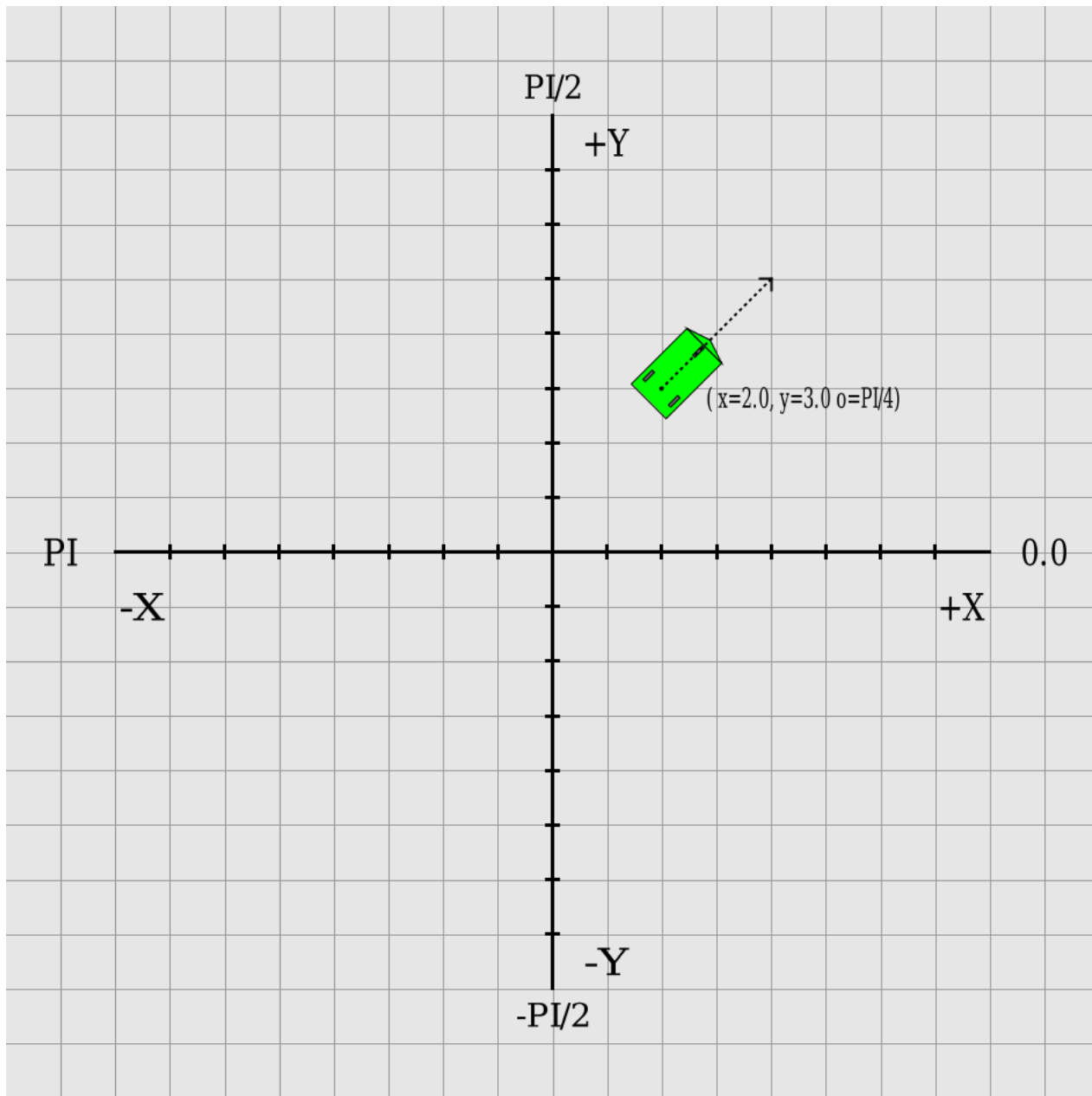
Figure 11 Coordinate system with sample AGV and orientation
